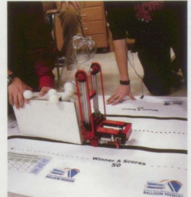
This robot has been programmed to follow the line on the paper that has been placed on the floor and dump the ping pong balls into the box at the end.
